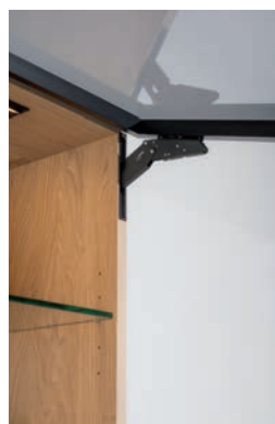
The door hinges are countersunk into the wooden element
